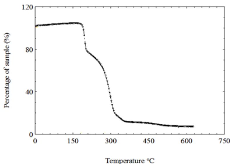
Figure 4. TGA thermograms of the synthesized disubstituted thiourea.
