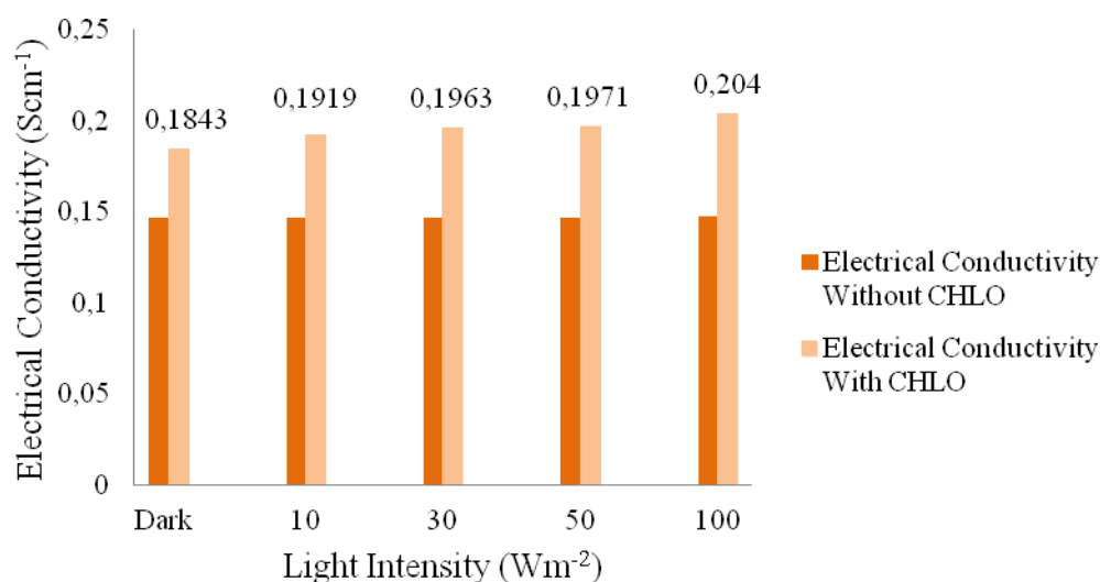
Figure 9. The electrical conductivity of ITO/TU/CHLO in both conditions with and without chlorophyll
