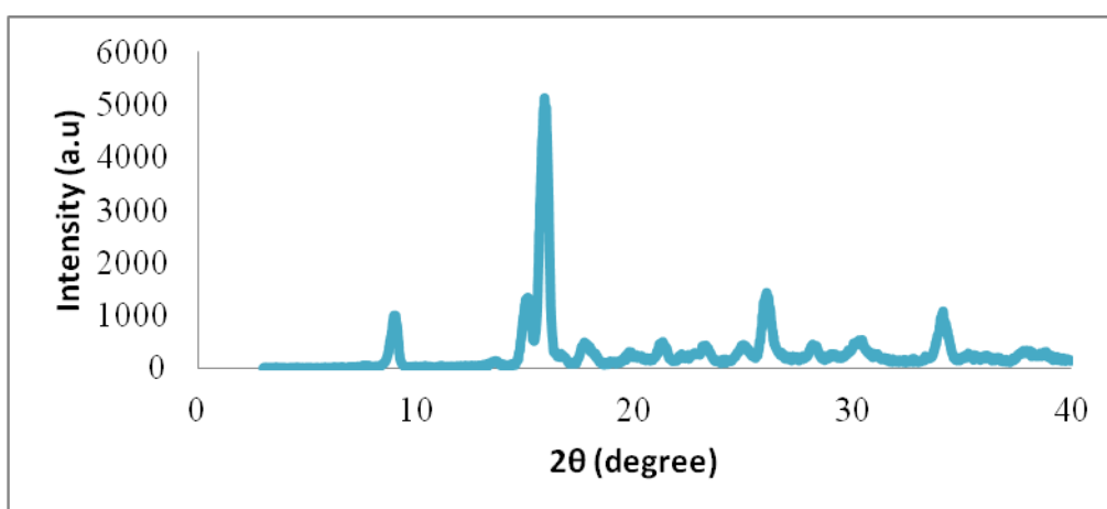
Figure 5. XRD pattern the synthesized compound.
