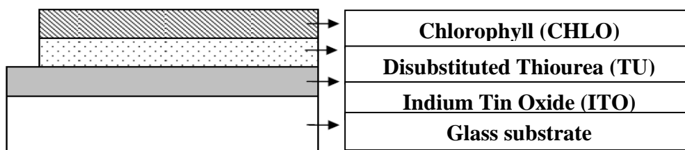
Figure 2. The general illustration of layer arrangement in thin film
