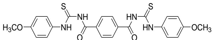
Figure 1. Molecular structure of disubstituted thiourea (TU) as active layer in photovoltaic cell synthesized in the study.
