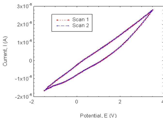
Figure 7. The cyclic voltammogram of disubstituted thiourea (TU) in \text{CH}_3\text{CN} on Pt electrode run at 0.05 V, 0.03 \text{ Vs}^{-1}
