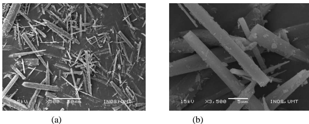
Figure 6. Surface morphology of the compound by (a) (500x magnification) and (b) (3,500x magnification).
