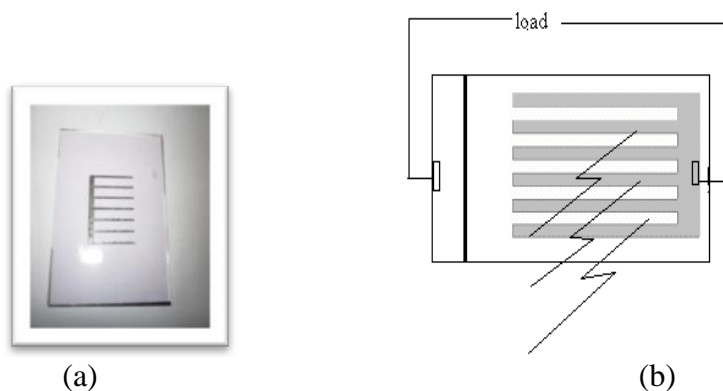
Figure 3. The schematic diagram (a) Thin film fabrication with aluminium grid (b) Solar cell under radiation of light
