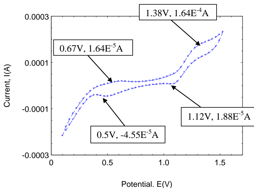
Figure 8. The cyclic voltammogram of disubstituted thiourea (TU) derivative ( 1 \times 10^{-5} M) in \text{CH}_3\text{CN} + 0.5 M sulphuric acid, 298 K at 0.05 V, 0.03 \text{Vs}^{-1}
