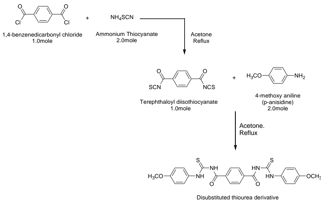
Scheme 1. General outline for synthesis of disubstituted thiourea (TU) derivative
