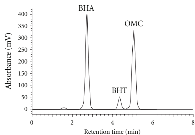
FIGURE 9: Chromatogram of BHA, BHT, and OMC in Elite hair oil sample using RP-HPLC-UV/Vis at \lambda_{\max} = 280 nm.
