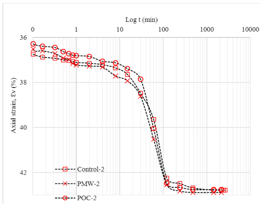
Fig. 8. Plot graph of \epsilon - \sigma_v' for specimens with thicknesses no- 2
