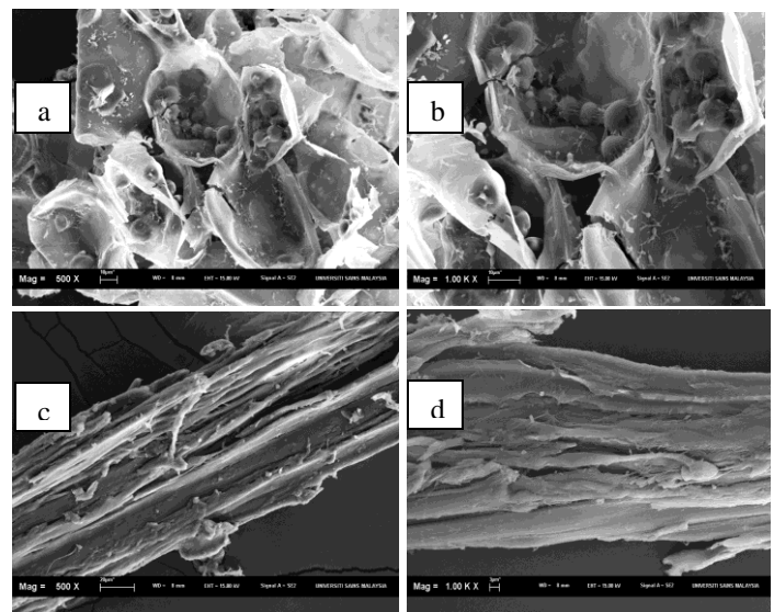
Figure 6. SEM micrographs of (a and b) parenchyma and (c and d) vascular bundle surface of oil palm trunk
