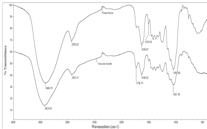
Figure 4. Infrared spectra of parenchyma and vascular bundle of oil palm trunk
