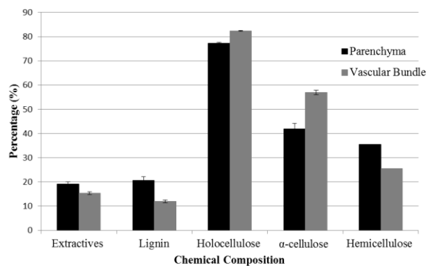
Figure 2. Chemical composition of parenchyma and vascular bundle of oil palm trunk
