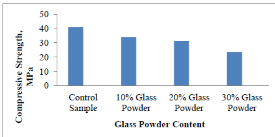
Figure 3: Compressive strength of 212 \mu\text{m} glass powder
