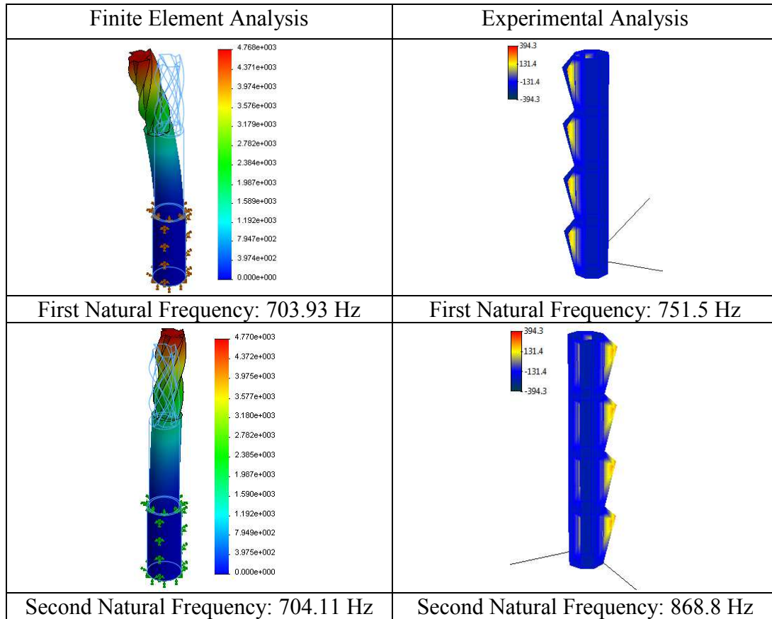
Fig.3: First two natural frequencies and mode shapes of cutting tool
