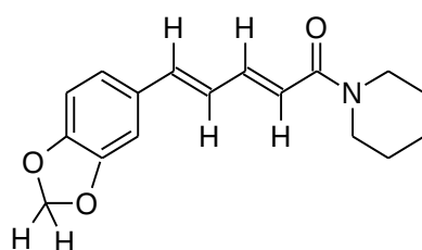
Figure 2.2: Molecular structure of piperidine
