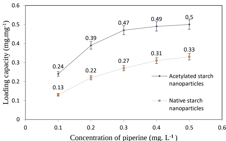
Figure 4.5: Loading capacity of piperine onto native starch nanoparticles and starch acetate nanoparticles, where n=3
