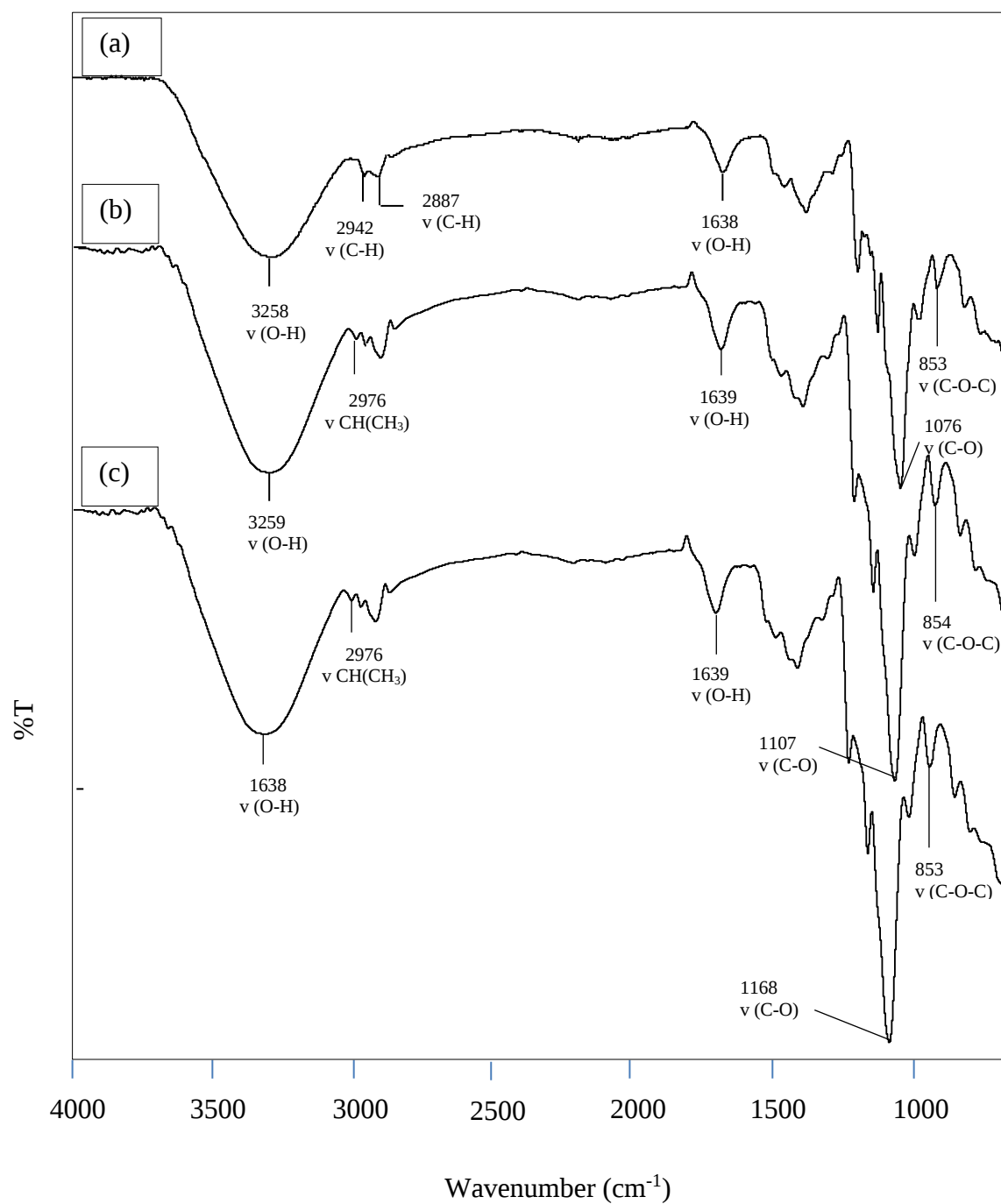
Figure 3.3: FTIR spectra of (a) native starch, (b) hydroxypropyl starch, and (c) hydroxypropyl starch nanoparticles
