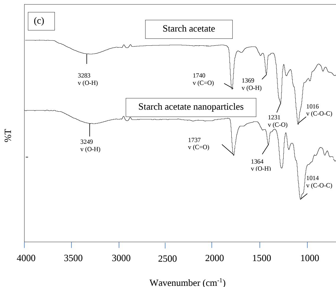
Figure 4.3: FTIR spectra of (a) starch acetate at various reaction durations (100°C reaction temperatures), (b) starch acetate at various reaction temperatures (20 minutes reaction time), and (c) starch acetate nanoparticles
