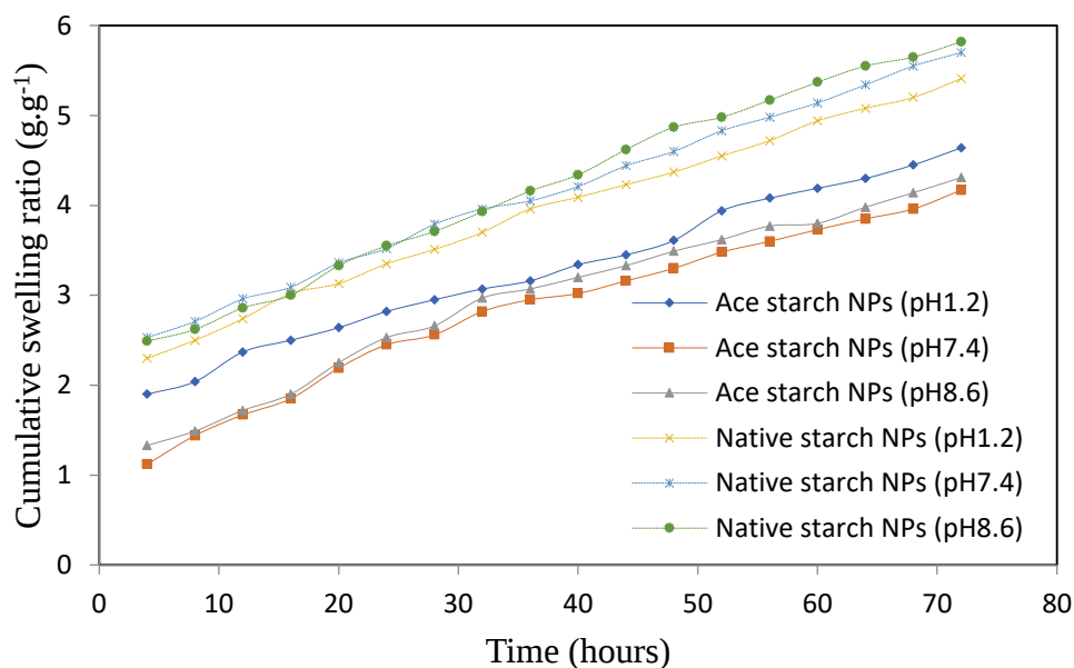
Figure 4.6: Swelling ratios of native starch nanoparticles and starch acetate nanoparticles in various pH of physiological media (1.2, 7.4 and 8.6) as a function of time
