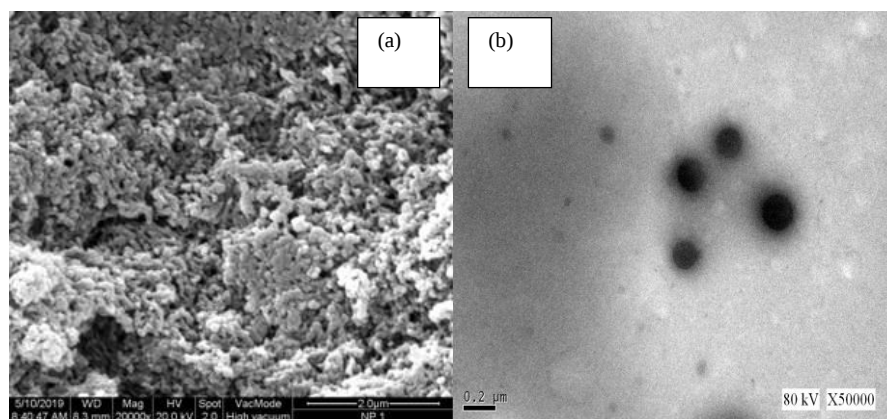
Figure 4.4: (a) FESEM images of starch acetate nanoparticles, and (b) TEM images of starch acetate nanoparticles
