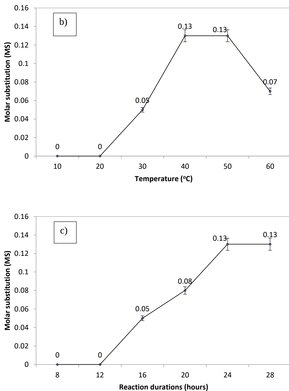
Figure 3.2: Effect of synthesis conditions on the molar substitution (MS) of hydroxypropyl starch (a) propylene oxide concentration (40 °C, 24 hours), (b) reaction temperatures (25% PO, 24 hours) and (c) reaction durations (25% PO, 40 °C), where n=3
