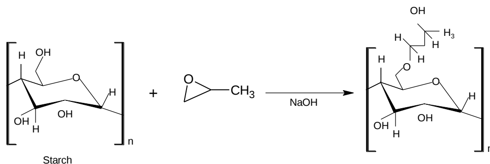
Figure 3.1: Reaction scheme of hydroxypropylation of native sago starch to form hydroxypropyl starch
