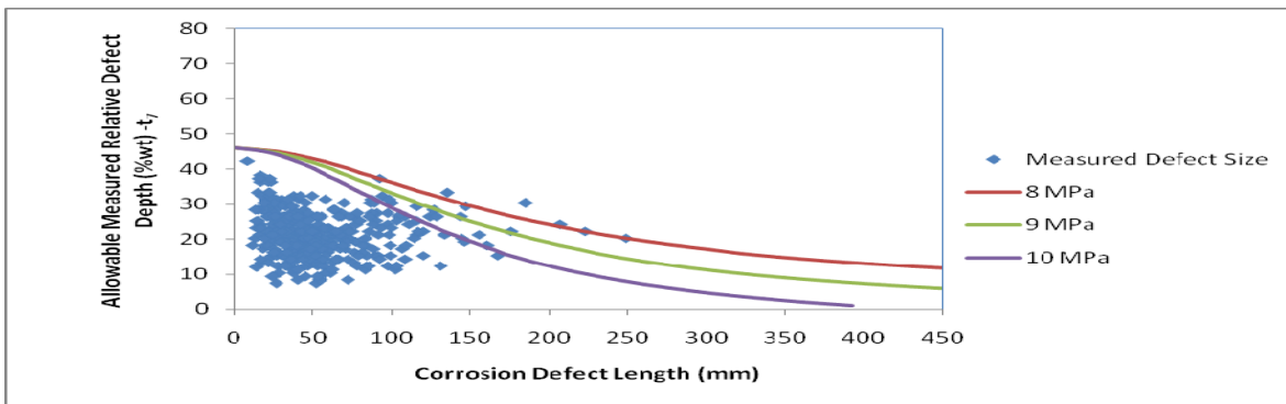
Figure 3: Projection of corrosion depth in year t_7 using DNV RP-F101 Assessment code
