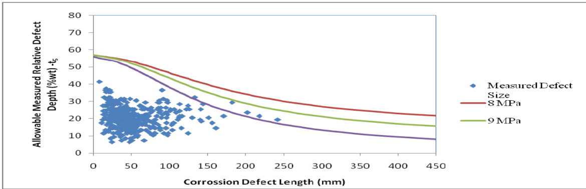
Figure 2: Projection of corrosion depth in year t_5 using DNV RP-F101 Assessment code
